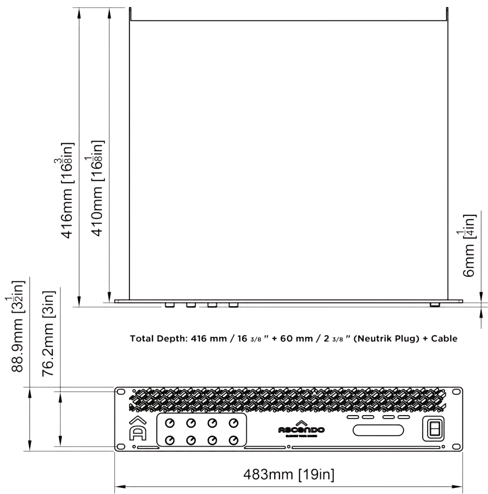
Figure 2. AIA8-2704 dimensions
