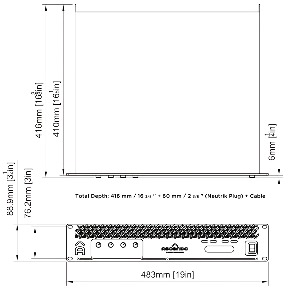
Figure 2. AIA4-6004 dimensions
