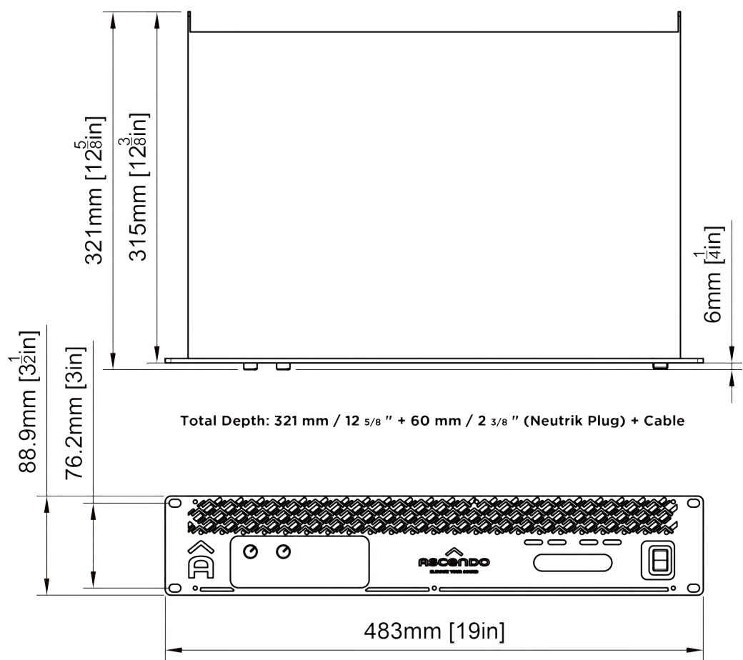
Figure 2. AIA2-6004 dimensions
